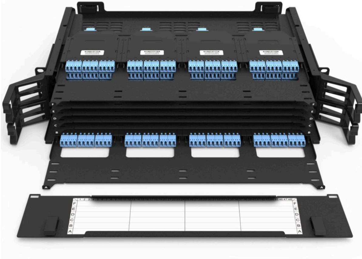
Top panel & door removed and tray shown extended.
