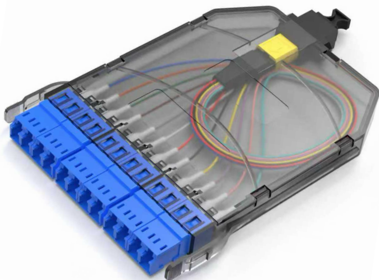
Part # 15588 Cassette, 12F LCupc - MPO
