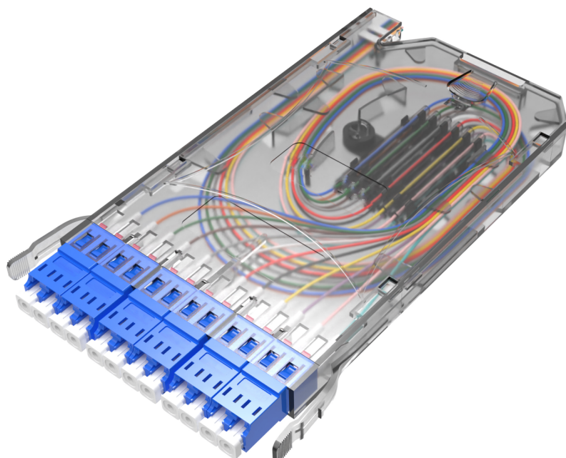
Part # 15583 Cassette, 12F LCupc OS2 Splice
